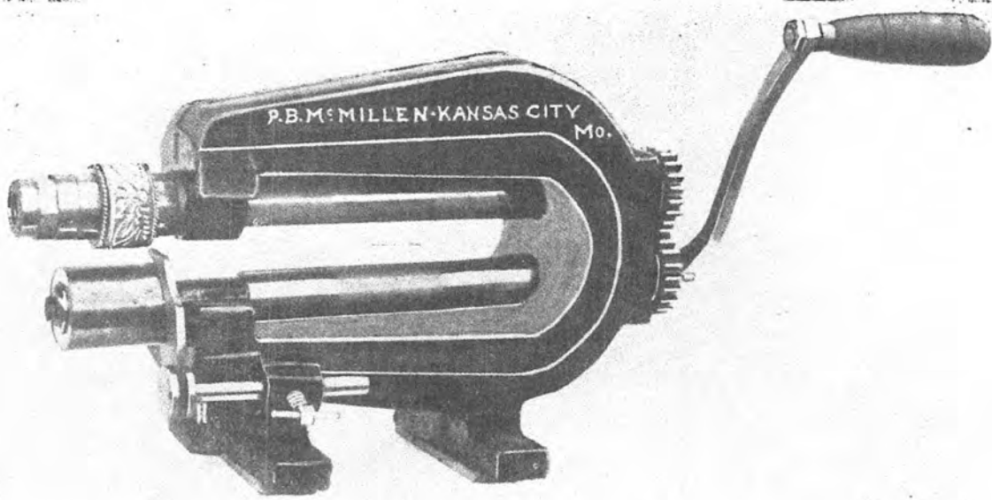
No. 926 Junior Embossing Machine
