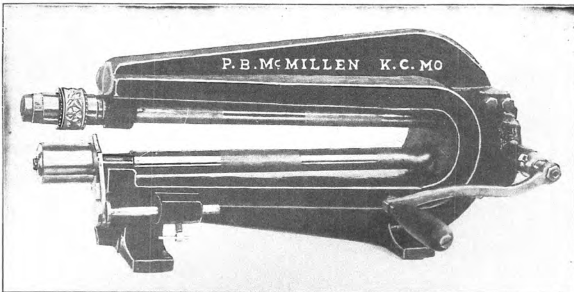
No. 934 McMillen's Saddle Embossing Machine. Takes 20 inches in the gap. The shafts are steel 1\frac{1}{4} inches in diameter; the spiral gears are steel; the cross screw has ball bearings; all other bearings are bronze. Prices are F.O.B. Kansas City, less embossing rolls.
